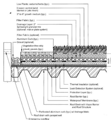
Figure 3: Typical Vegetated Roof Section
